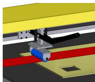
Roller Polishing Attachment
